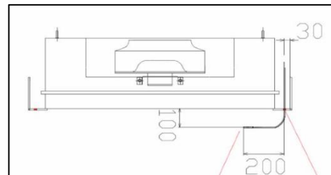
Figures 5a & 5b – Recommended Cleanroom T&H Probe Mounting Location
