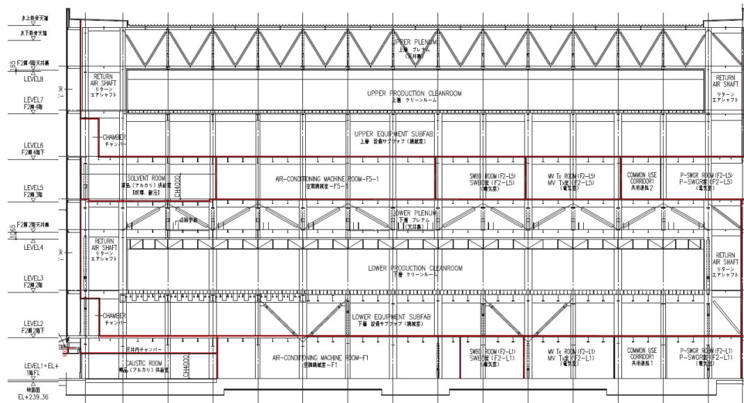
Figure 2 – Typical Double-Level FAB with 8 Levels (2-Levels of FAB Cleanroom)
