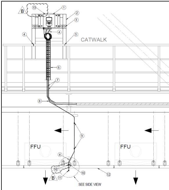
Figure 4 – Example Cleanroom T&H Transmitter and Probe Mounting Detail
